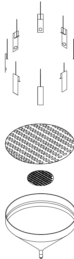
12" Rain Gauge
